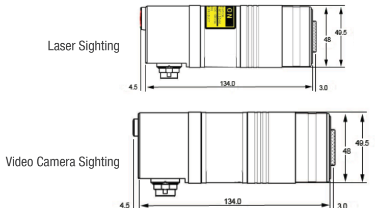
Product Dimensions in mm
