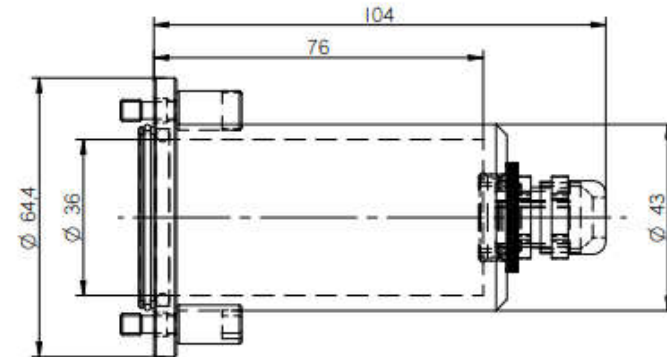
Protective End Cap for Cooling Jacket 40,42,44 series P/N PSC-3310A23015
